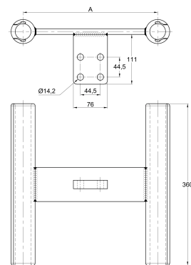
2D DRAWING · DIMENSIONS (MM)
