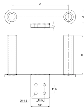
2D DRAWING · DIMENSIONS (MM)
