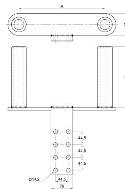
2D DRAWING · DIMENSIONS (MM)
