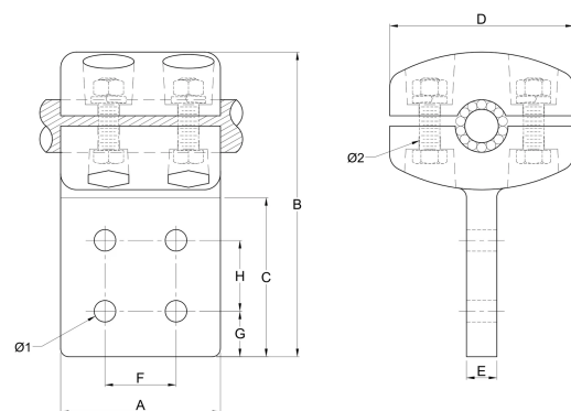
2D DRAWING · DIMENSIONS (MM)
