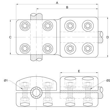
2D DRAWING · DIMENSIONS (MM)
