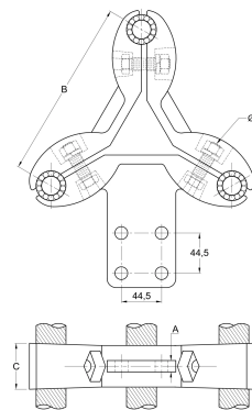
2D DRAWING · DIMENSIONS (MM)
