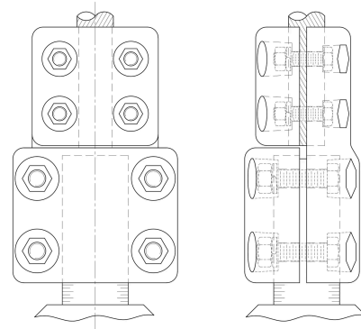
2D DRAWING · DIMENSIONS (MM)
