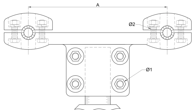
2D DRAWING · DIMENSIONS (MM)
