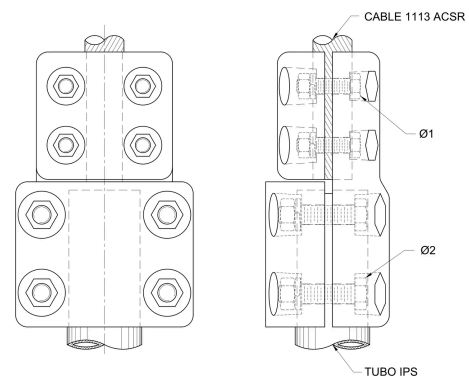
2D DRAWING · DIMENSIONS (MM)
