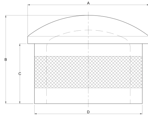
2D DRAWING · DIMENSIONS (MM)
