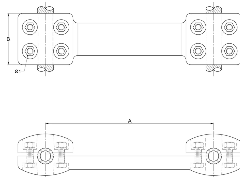
2D DRAWING · DIMENSIONS (MM)
