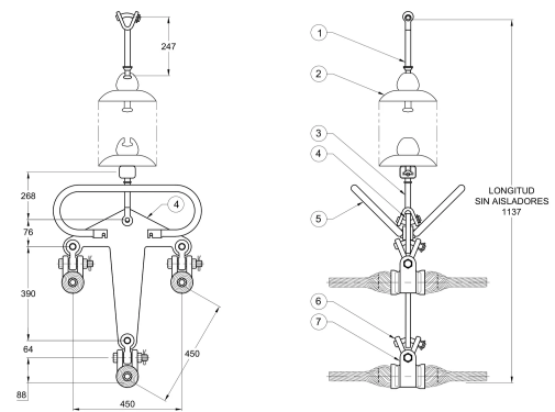
2D DRAWING · DIMENSIONS (MM)
