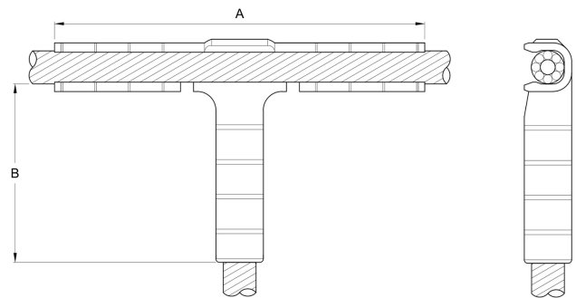
2D DRAWING · DIMENSIONS (MM)
